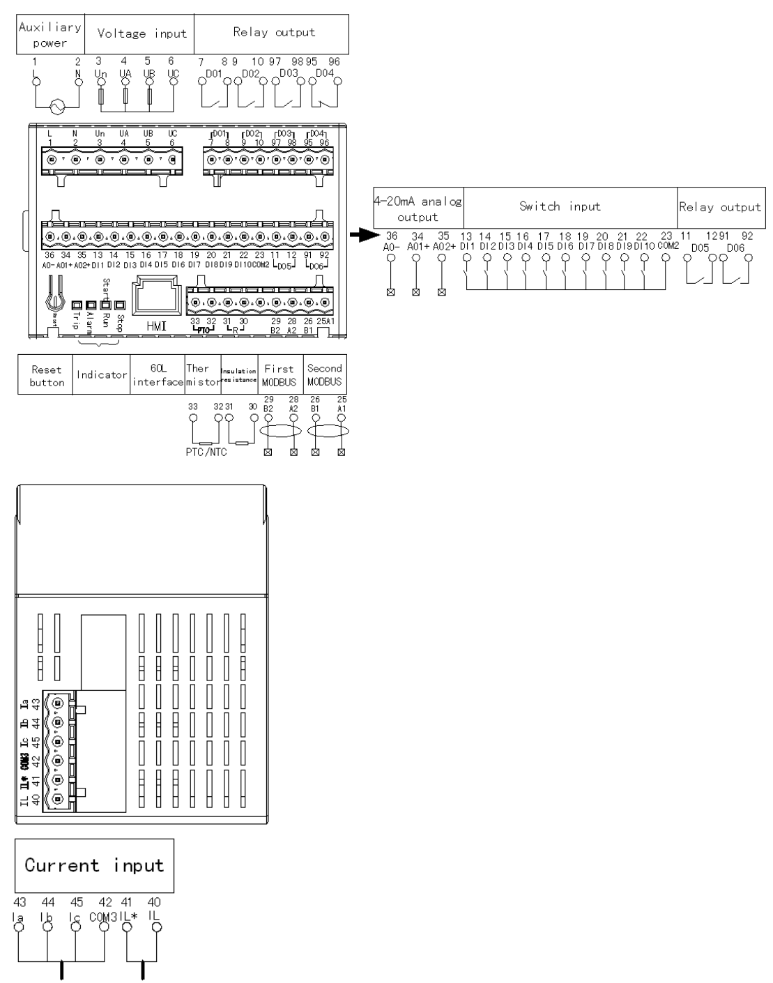
FIG. 13 ARD3M terminal arrangement
